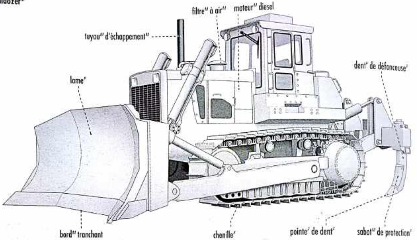
bulldozer m
